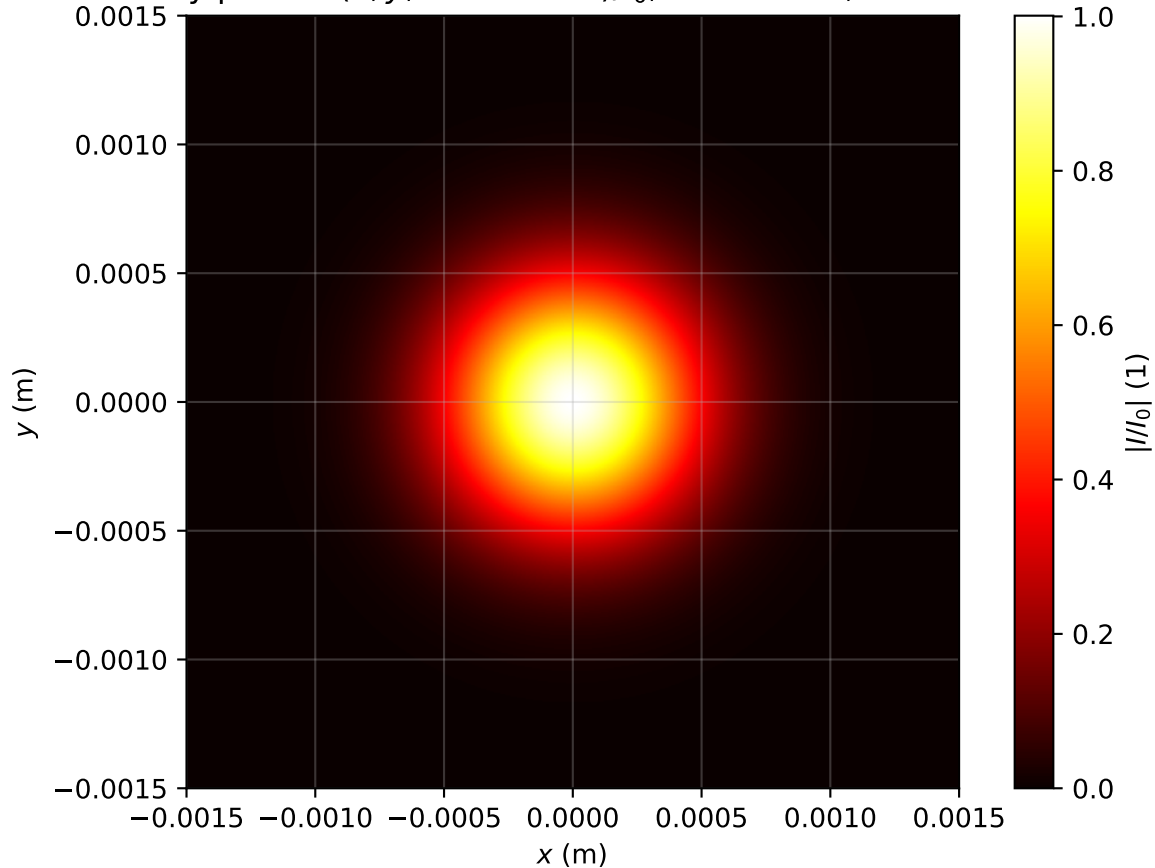
Intensity profile I(x, y, z = 0.080m)/I_0 , Pin=0.4Pcr, artificial time
